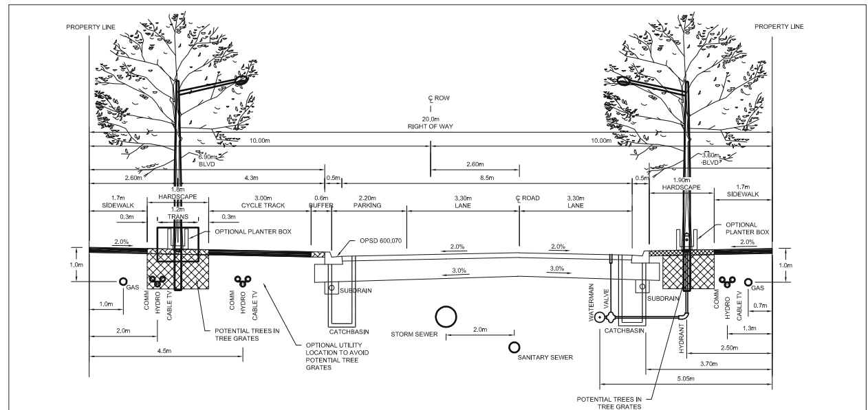
20.0m Minor Collector Road (Character) Section (In Node)
