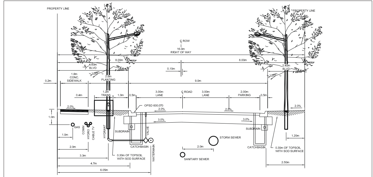
16.0m Local Road Section
