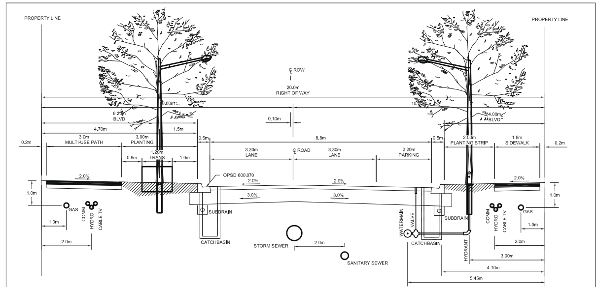
20.0m Minor Collector Road (Character) Section (Outside Node - Condition A)
