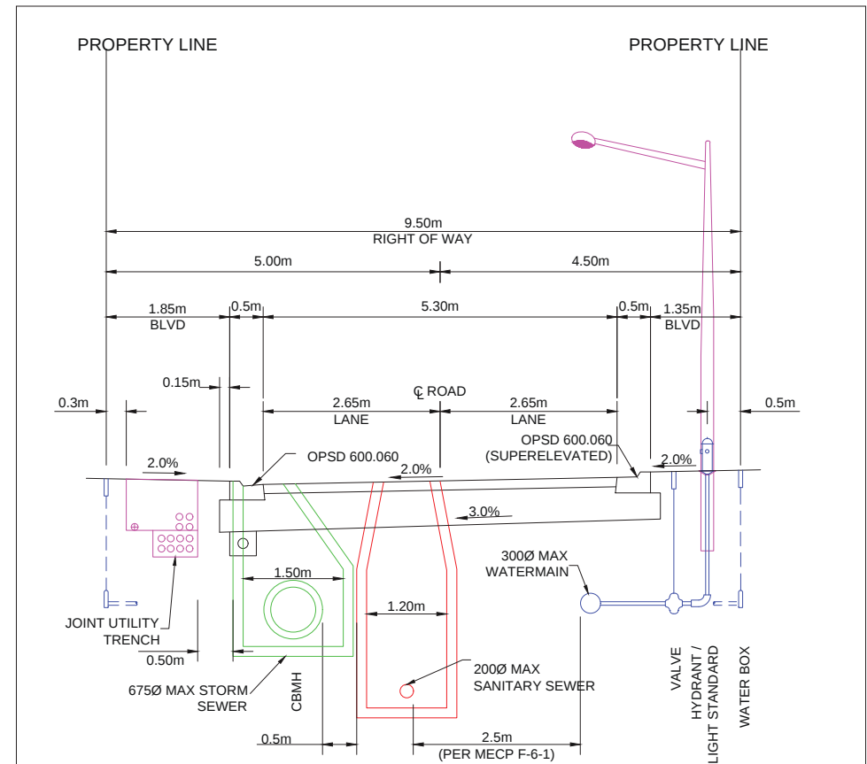
9.5m Laneway Section
