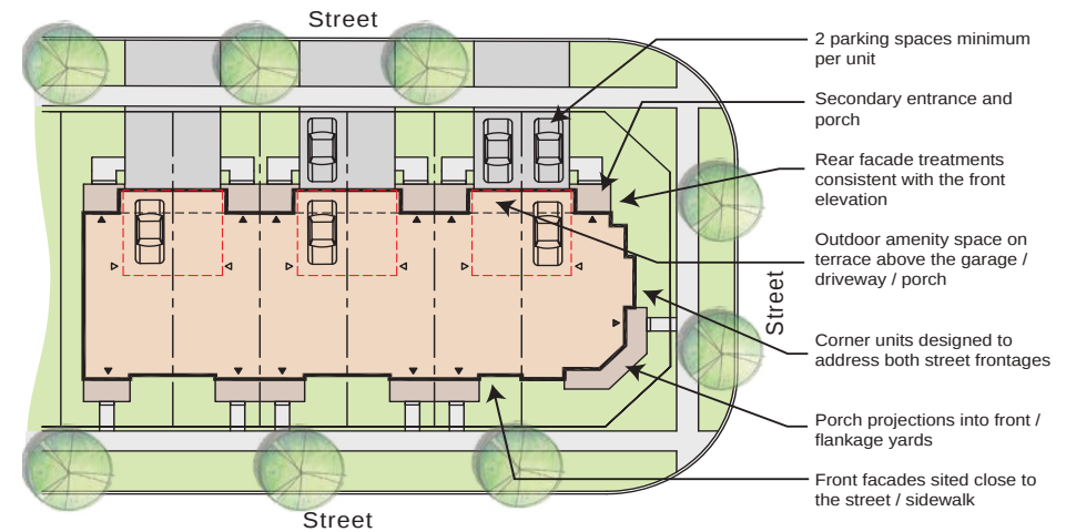
Conceptual Demonstration Site Plan for Dual Frontage Townhouses
