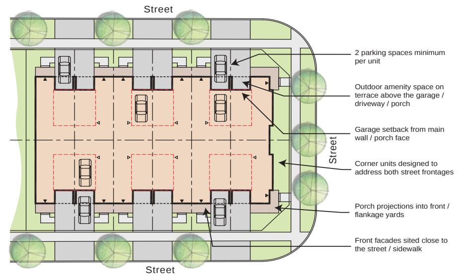
Conceptual Demonstration Site Plan for Back-to-Back Townhouses
