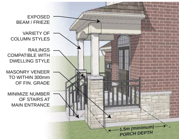
Typical porch detail
