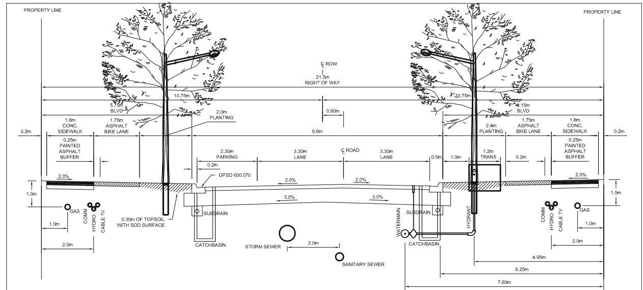
21.5m Minor Collector Road Section
