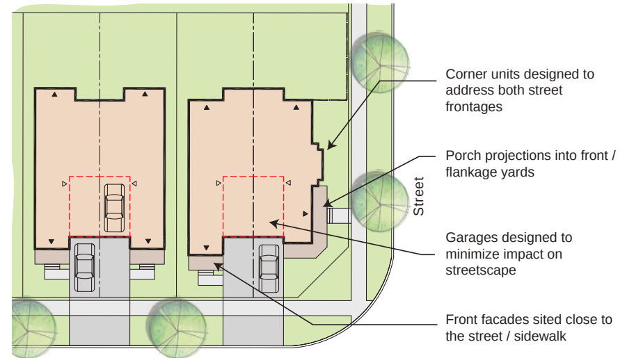
Conceptual Demonstration Site Plan For Semi-Detached Dwellings
