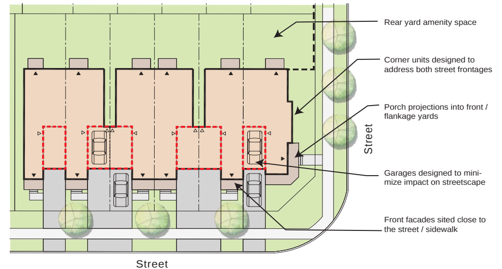
Conceptual Demonstration Site Plan for Street Townhouses
