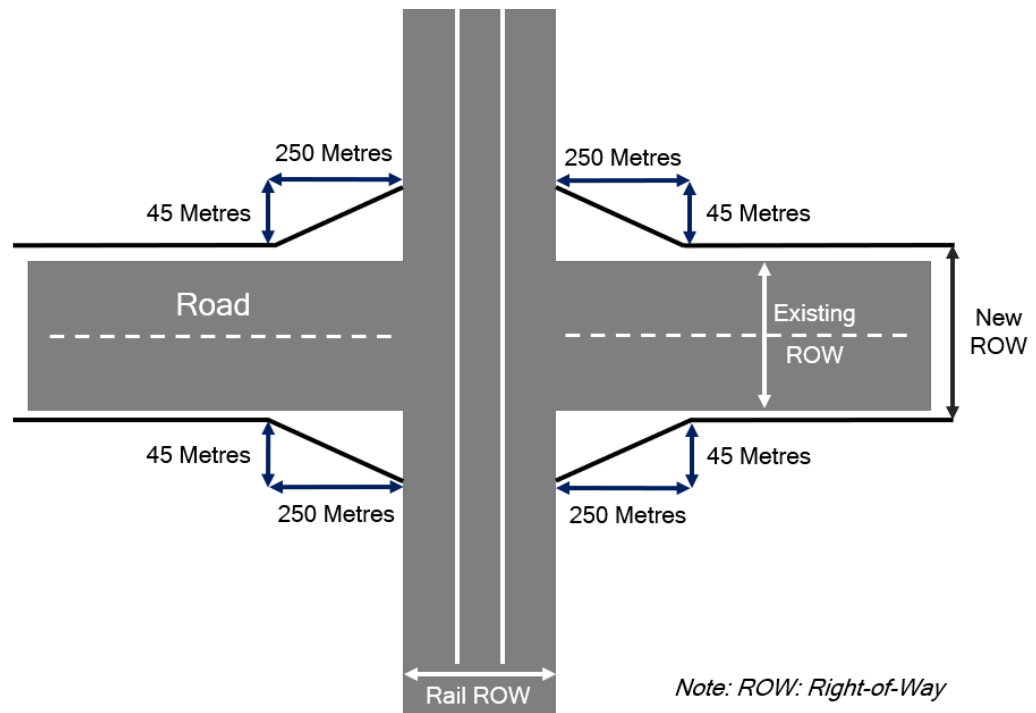
Figure 6. Minimum Right of Way Requirements For Future Railway Grade Separations.
